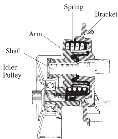
Cross Section
